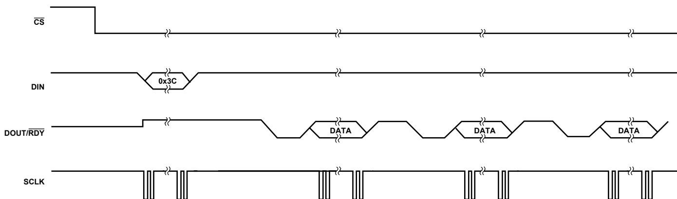
Figure 13. Continuous Read
