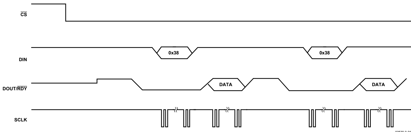
Figure 12. Continuous Conversion
