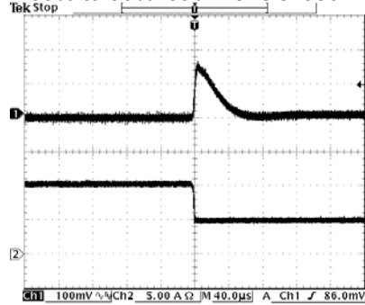
100% to 50% load Transient at V_{in}=5 V, V_o=3.3 V
