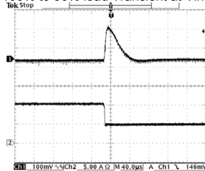
100% to 50% load Transient at V_{in}=12 V, V_o=0.75 V
