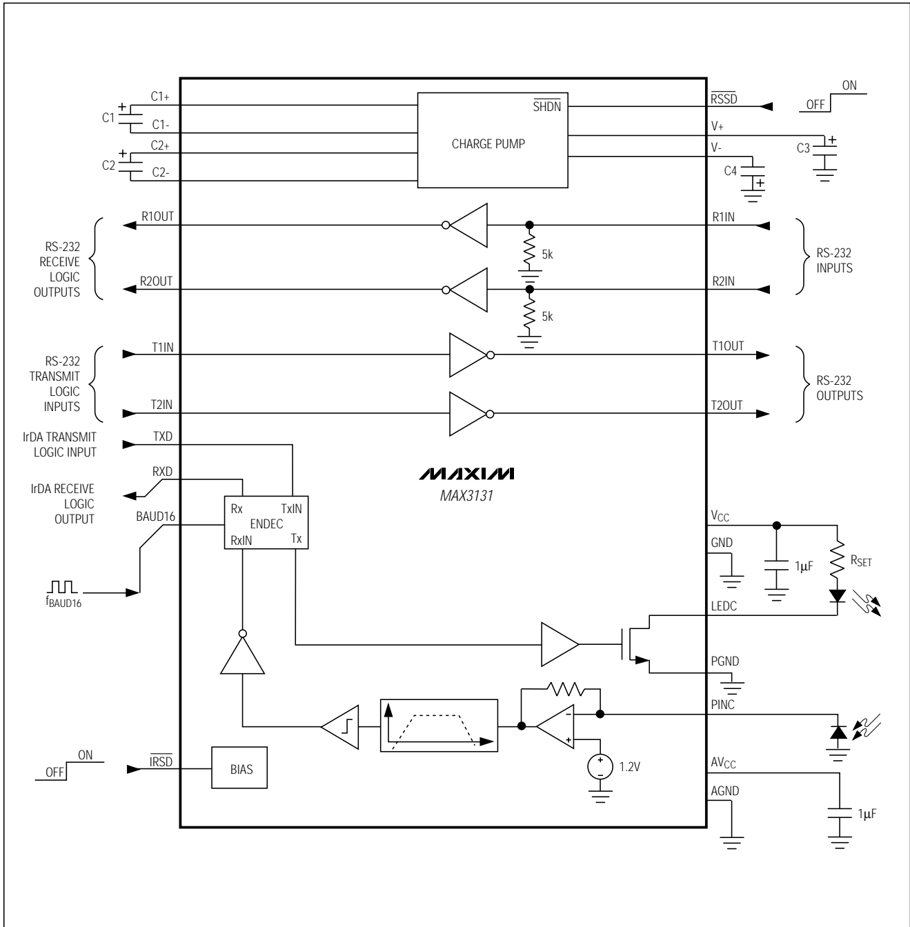
Figure 2. MAX3131 Functional Diagram
