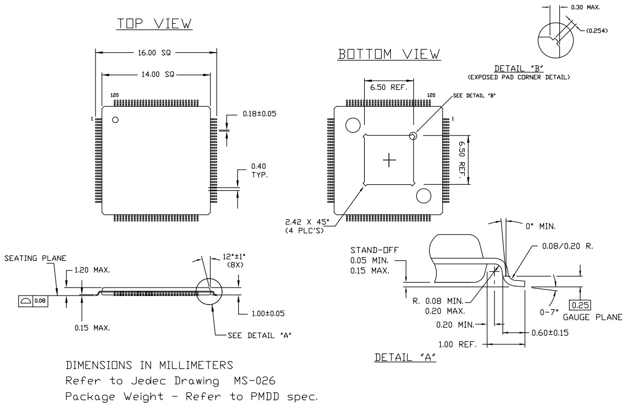
Figure 18. 120-pin TQFP (14 × 14 × 1.0 mm) AE120A (6.5 × 6.5 E-Pad) Package Outline, 001-48723
