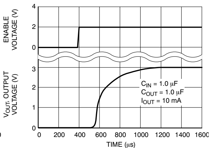
Figure 11. Turn-On Response
