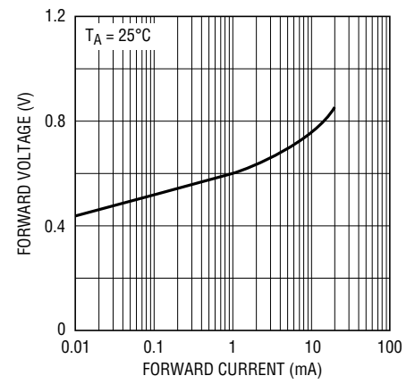
Forward Characteristics
