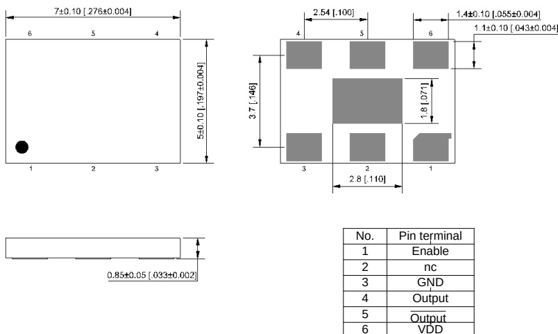
External Dimensions units: mm[inch]
