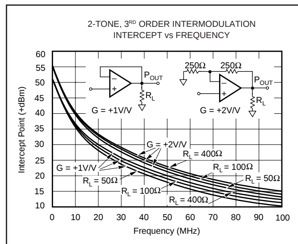
FIGURE 9. 2-Tone, 3rd Order Intermodulation Intercept vs Frequency.
