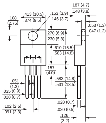
TO-220
