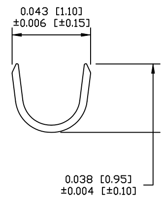
DETAIL A - A
