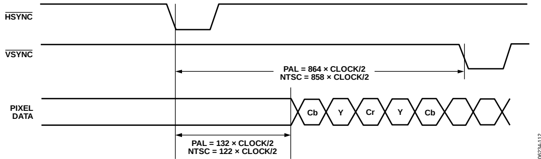
Figure 114. SD Timing Mode 2, Odd-to-Even Field Transition (Master/Slave)
