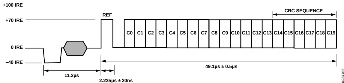
Figure 95. Standard Definition CGMS Waveform
