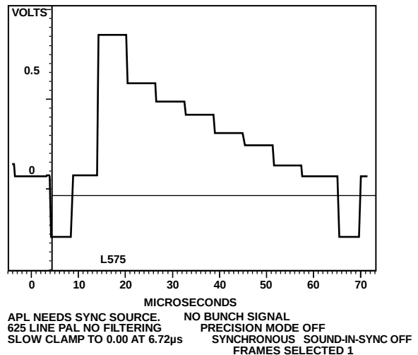
Figure 136. PAL Luma
