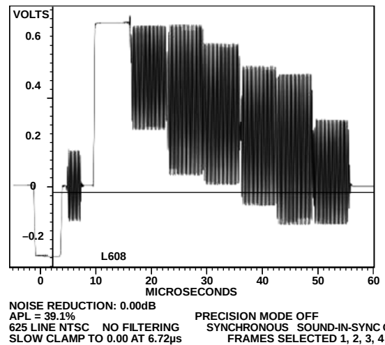
Figure 135. PAL Color Bars (75%)
