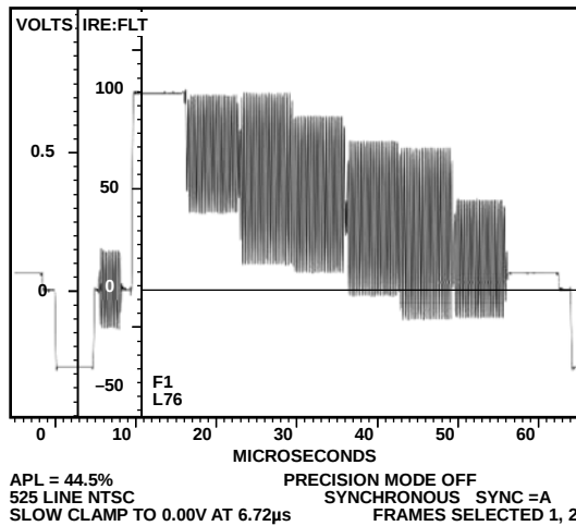
Figure 132. NTSC Color Bars (75%)
