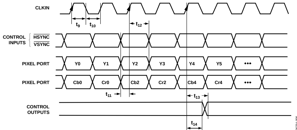
Figure 7. ED/HD-SDR Input, 16-Bit 4:2:2 YCrCb, Input Mode 001
