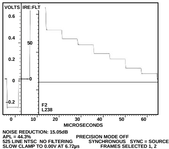
Figure 133. NTSC Luma
