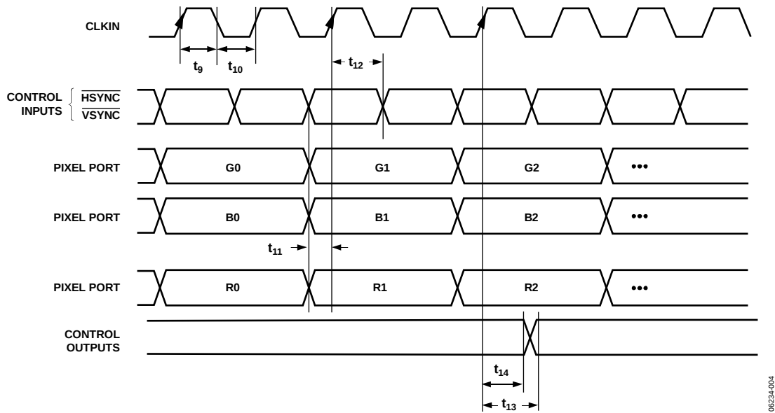
Figure 6. SD Input, 16-Bit 4:4:4 RGB, Input Mode 000
