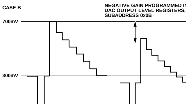
Figure 70. Programmable DAC Gain—Positive and Negative Gain
