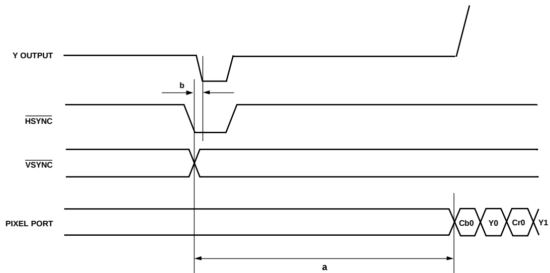
Figure 12. ED-SDR, 16-Bit 4:2:2 YCrCb ( \overline{\text{HSYNC}}/\overline{\text{VSYNC}} ) Input Timing Diagram
