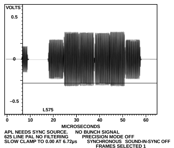
Figure 137. PAL Chroma
