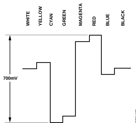
Figure 122. Pr Levels—PAL
