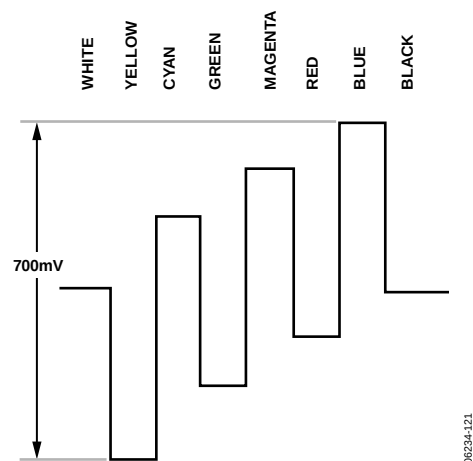
Figure 123. Pb Levels—PAL
