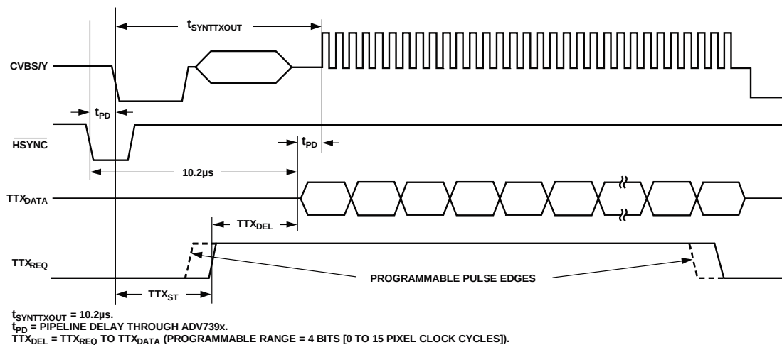
Figure 86. Teletext Functionality Diagram
