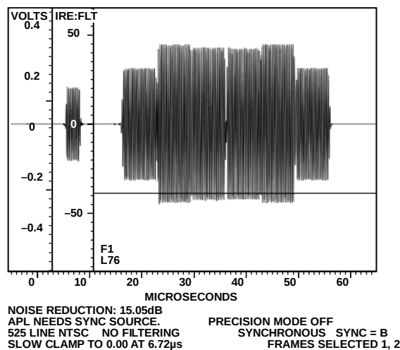
Figure 134. NTSC Chroma
