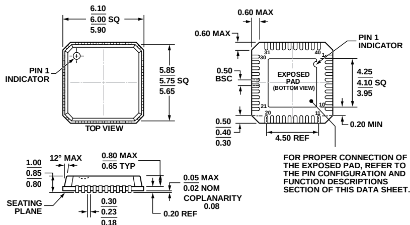
Figure 147. 40-Lead Lead Frame Chip Scale Package [LFCSP_VQ] 6 mm × 6 mm Body, Very Thin Quad (CP-40-1)
