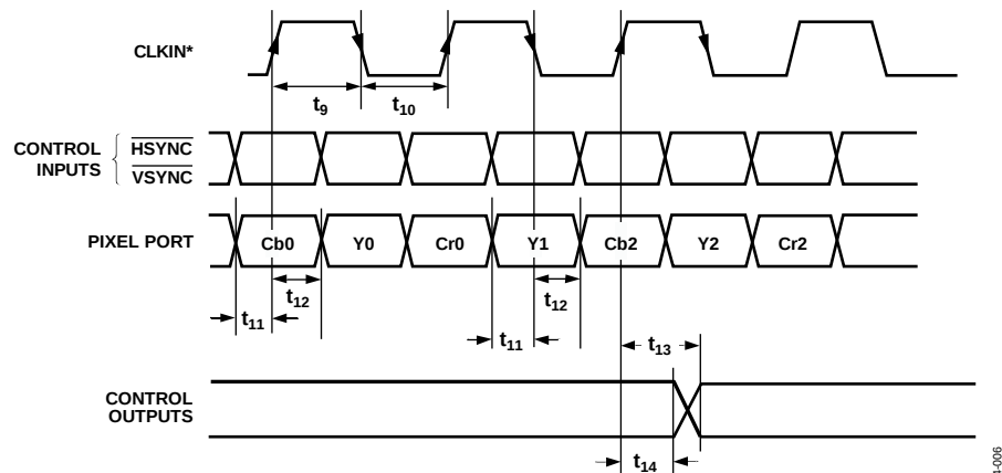
Figure 8. ED/HD-DDR Input, 8-/10-Bit 4:2:2 YCrCb (HSYNC/VSYNC), Input Mode 010
