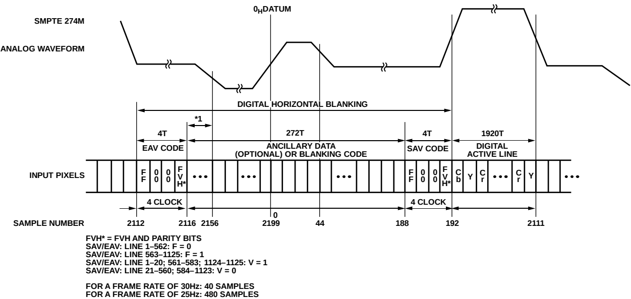
Figure 138. EAV/SAV Input Data Timing Diagram (SMPTE 274M)
