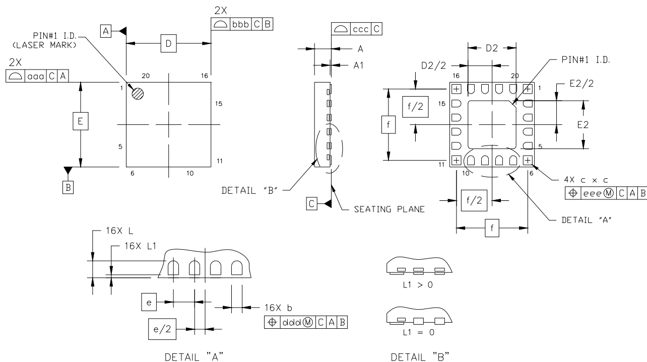
Figure 12. 20-Pin Quad Flat No-Lead (QFN)
