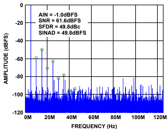
FIGURE 19. SINGLE-TONE SPECTRUM AT 995MHz
