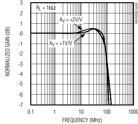
MEDIUM-SIGNAL FREQUENCY RESPONSE
