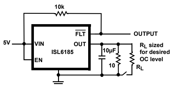
FIGURE 29B. CURRENT LIMITING
