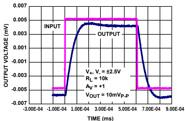
FIGURE 7. SMALL SIGNAL TRANSIENT RESPONSE
