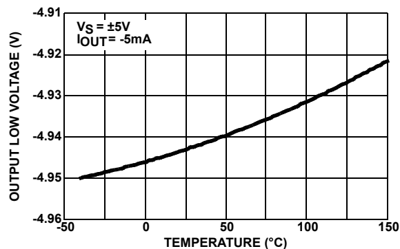
FIGURE 7. OUTPUT LOW VOLTAGE vs TEMPERATURE
