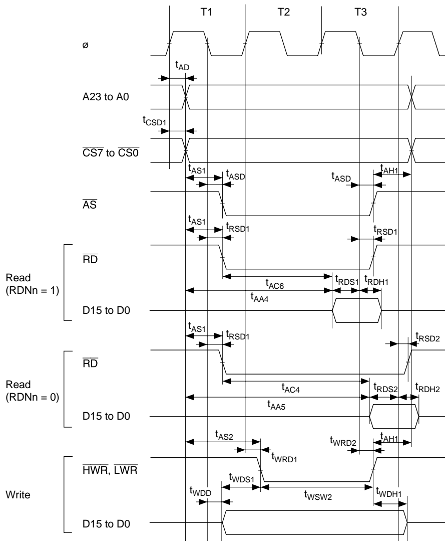
Figure 21.7 Basic Bus Timing: Three-State Access
