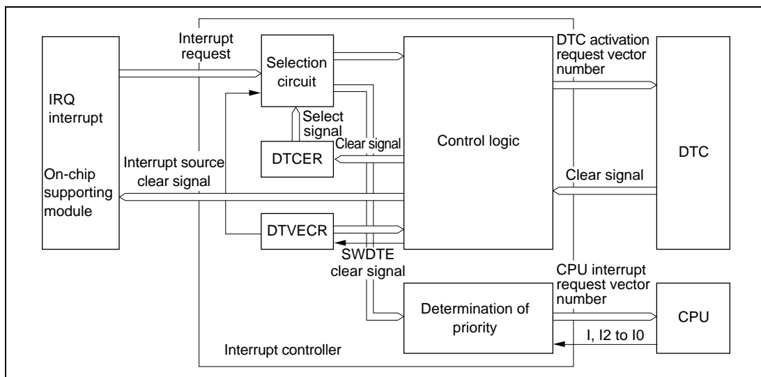
Figure 5.6 DTC, DMAC, and Interrupt Controller
