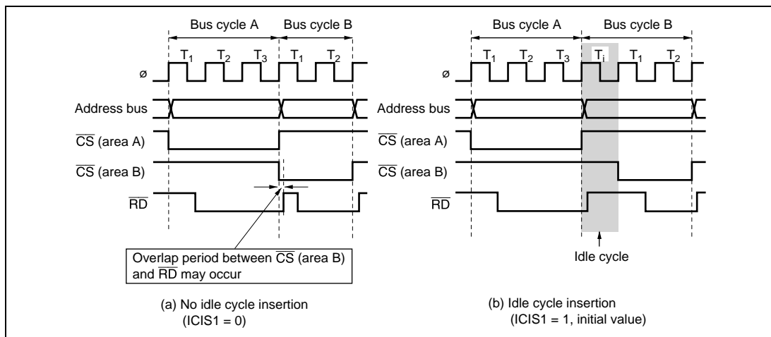
Figure 6.22 Relationship between Chip Select ( \overline{\text{CS}} ) and Read ( \overline{\text{RD}} )
