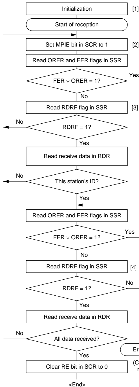
Figure 13.13 Sample Multiprocessor Serial Reception Flowchart (1)
