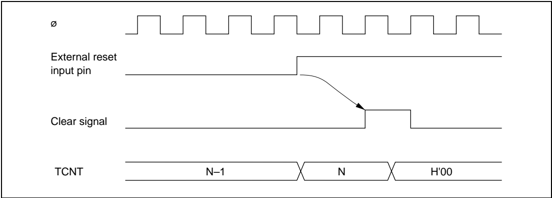
Figure 11.8 Timing of Clearance by External Reset
