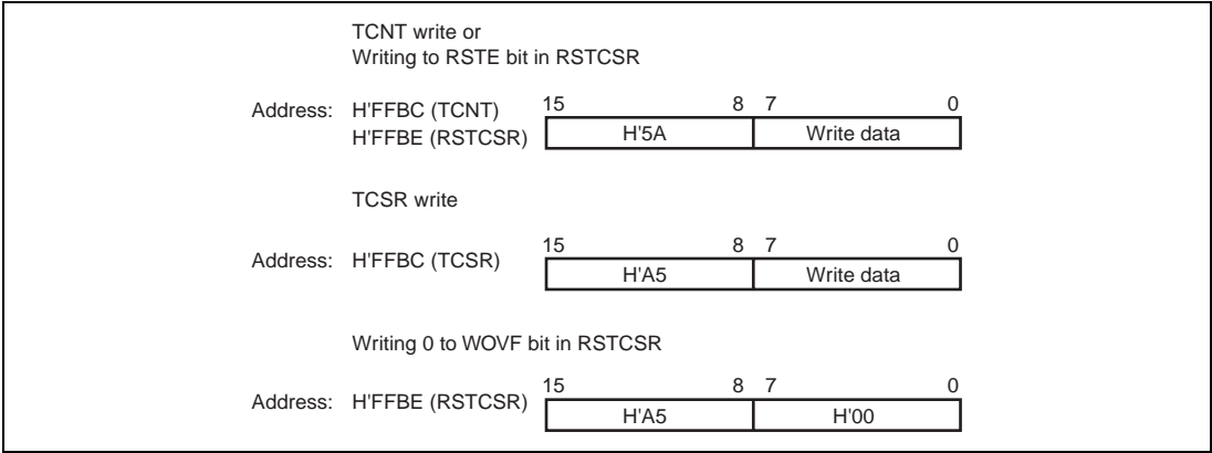
Figure 12.4 Writing to TCNT, TCSR, and RSTCSR
