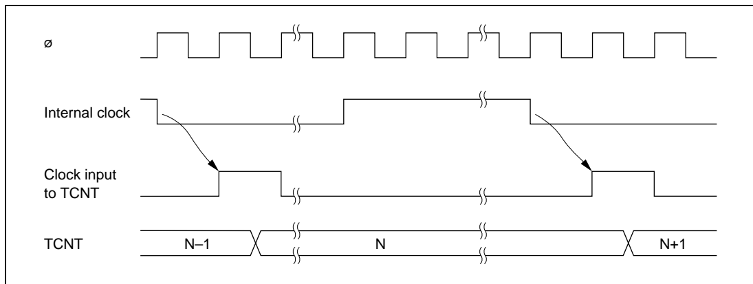
Figure 11.3 Count Timing for Internal Clock Input
