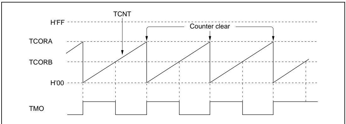
Figure 11.2 Example of Pulse Output
