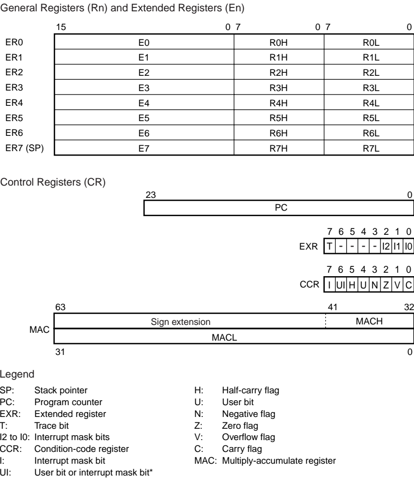
Figure 2.6 CPU Registers
