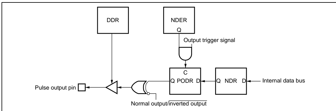
Figure 10.2 Overview Diagram of PPG
