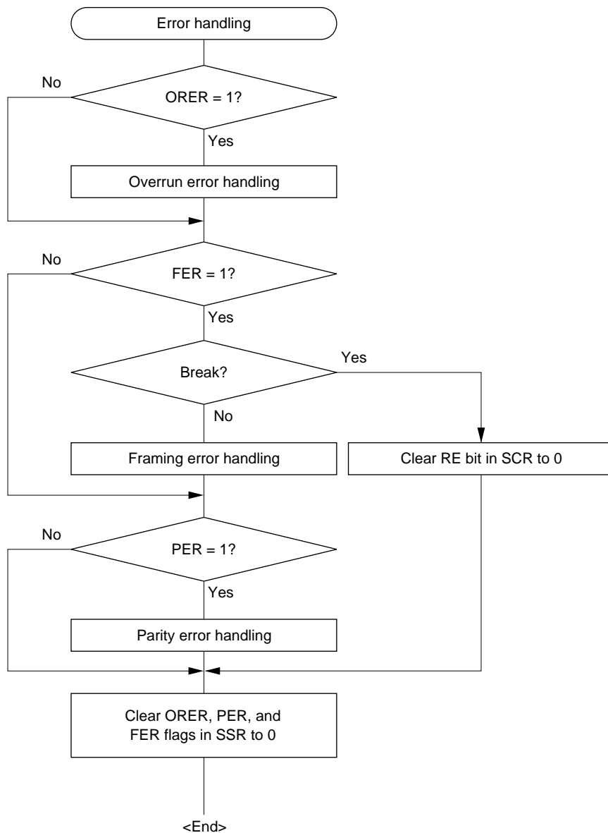
Figure 13.9 Sample Serial Reception Data Flowchart (2)
