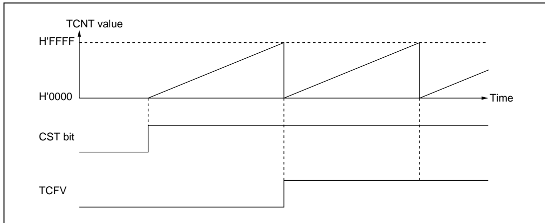
Figure 9.3 Free-Running Counter Operation
