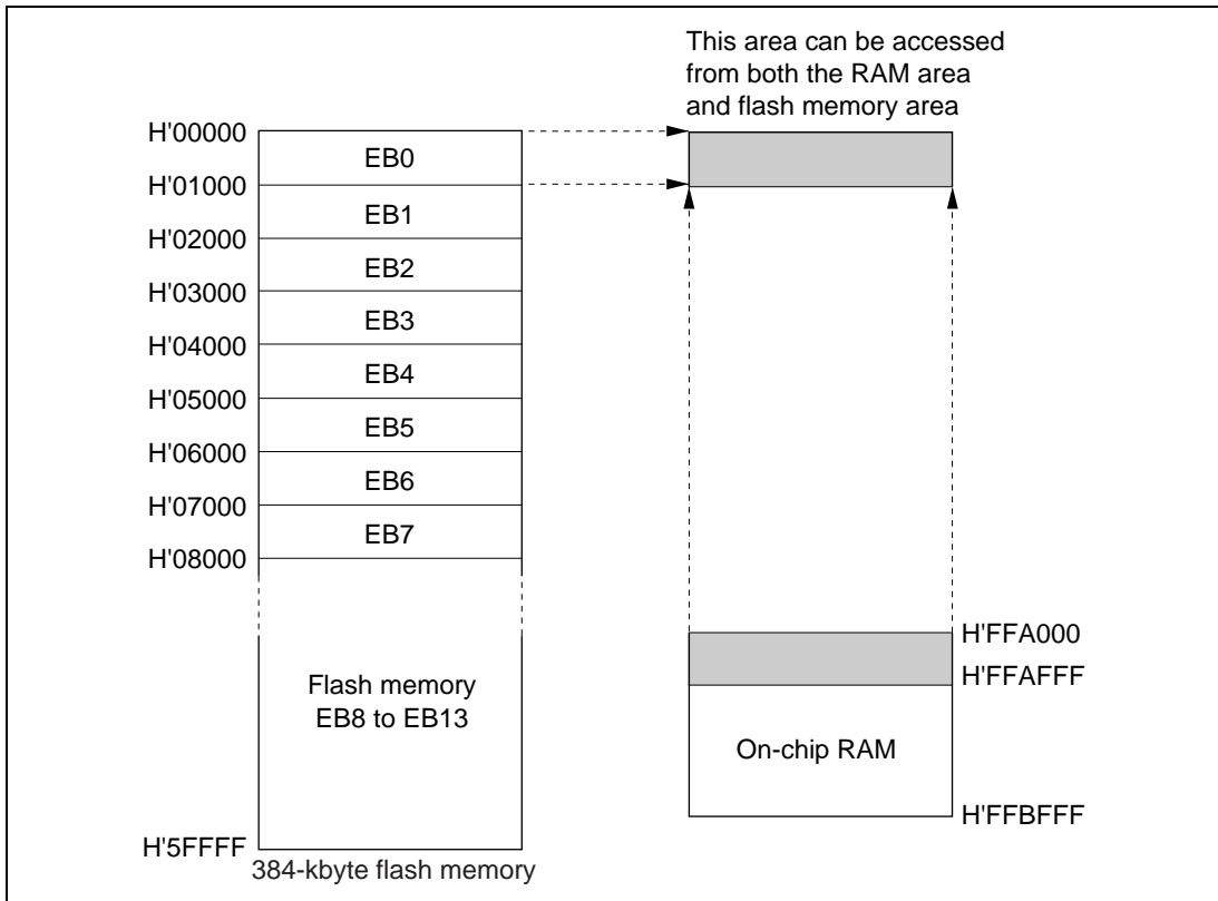
Figure 17.8 Example of RAM Overlap Operation
