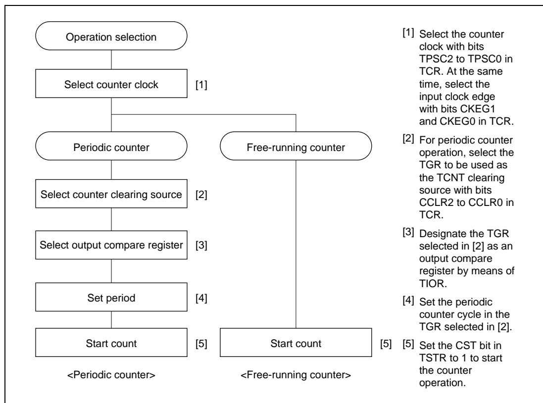
Figure 9.2 Example of Counter Operation Setting Procedure
