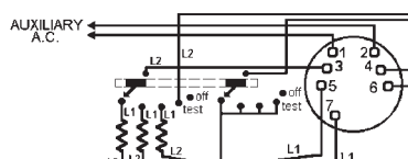
Fig. 17 Models 077-45R, 078-45R Temperature Indicator for Resistance Temperature Detector (RTD).
