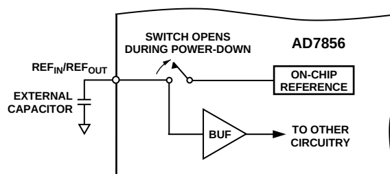
Figure 23. On-Chip Reference During Power-Down
