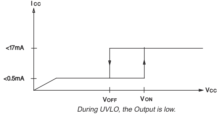
Figure 6-3. Undervoltage Lockout
