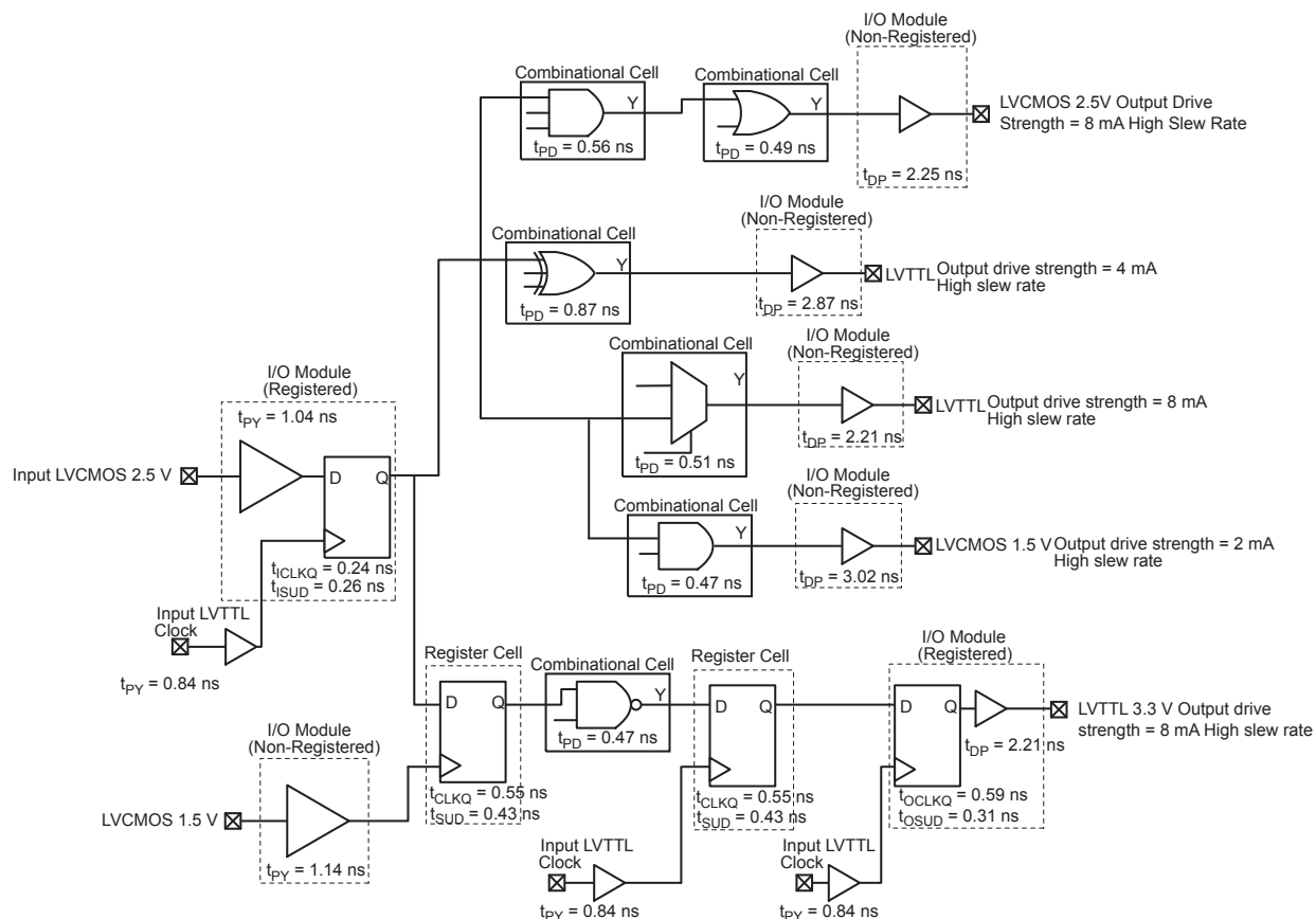
Figure 2-2 • Timing Model
