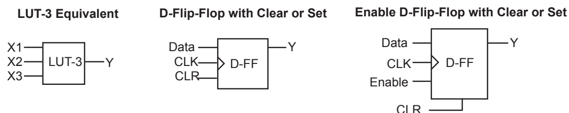
Figure 1-5 • VersaTile Configurations
