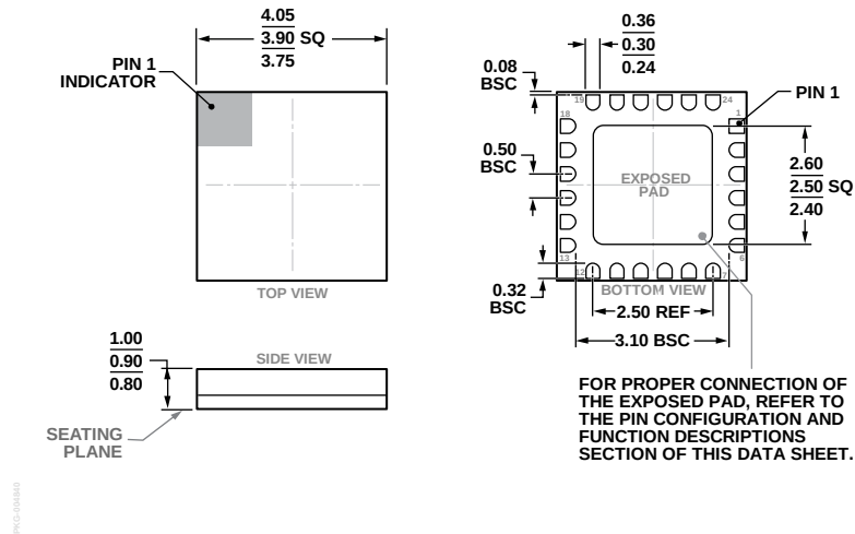
Figure 83. 24-Terminal Ceramic Leadless Chip Carrier [LCC] (E-24-1) Dimensions shown in millimeters
