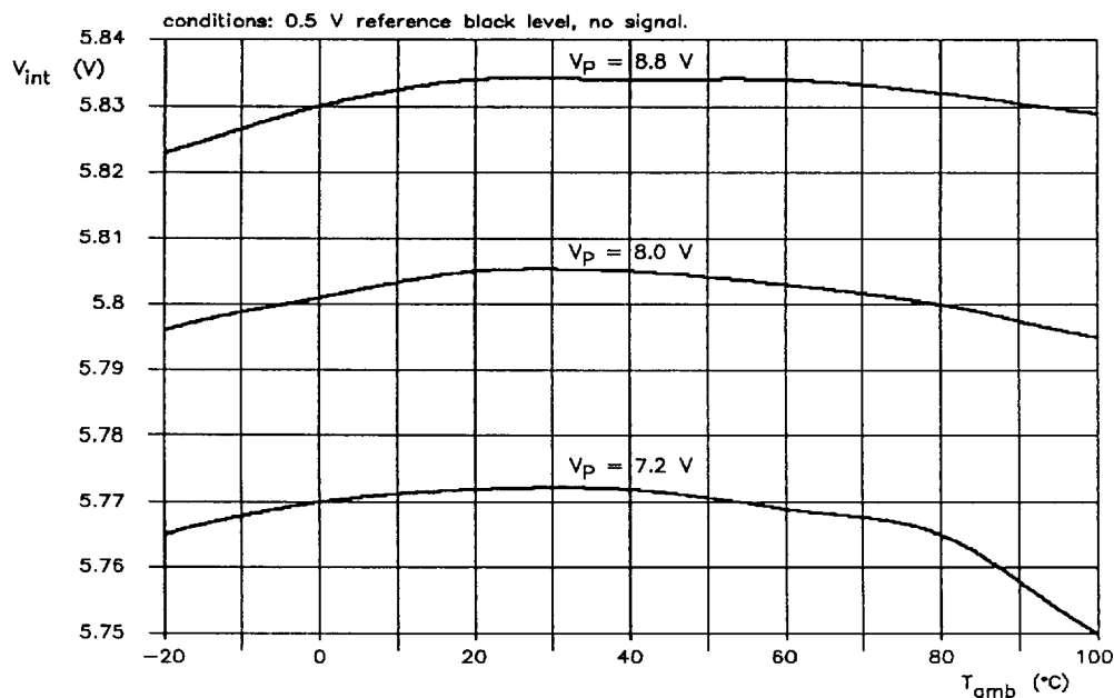
Fig.8 Typical variation of V_{Int} with temperature and power supply voltage.
