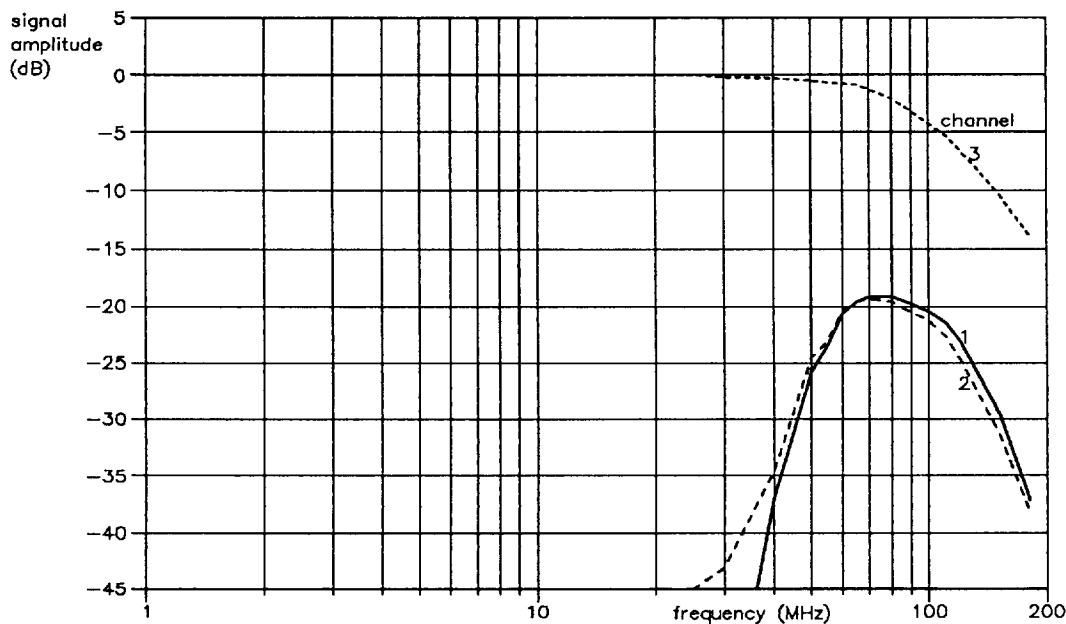
Fig.15 Typical crosstalk: Channel 3 → 1 and 2.
