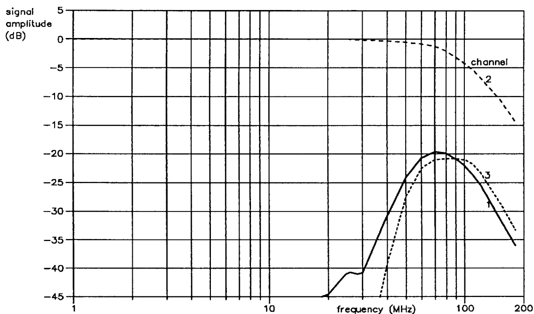
Fig.14 Typical crosstalk: Channel 2 → 1 and 3.
