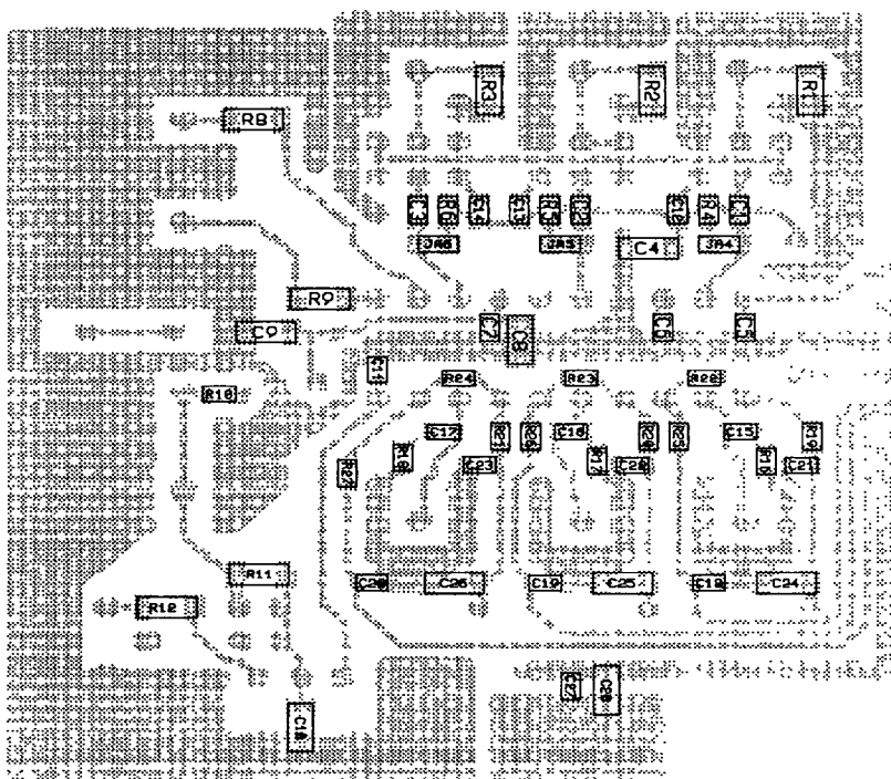
Fig.18 Double sided test PCB layout.
