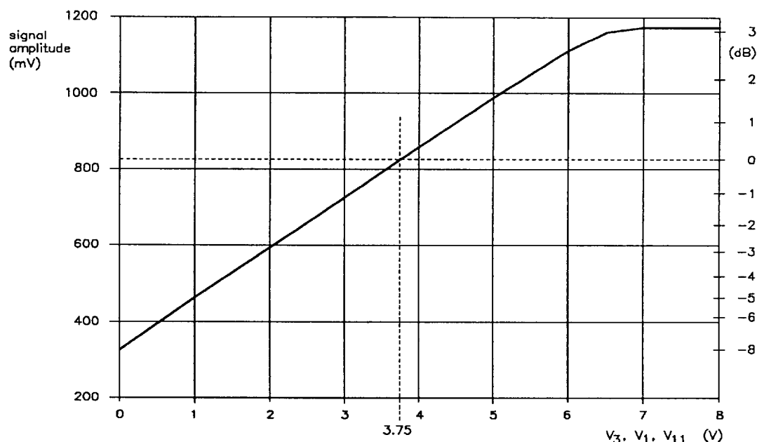
Fig.7 Typical gain characteristic.
