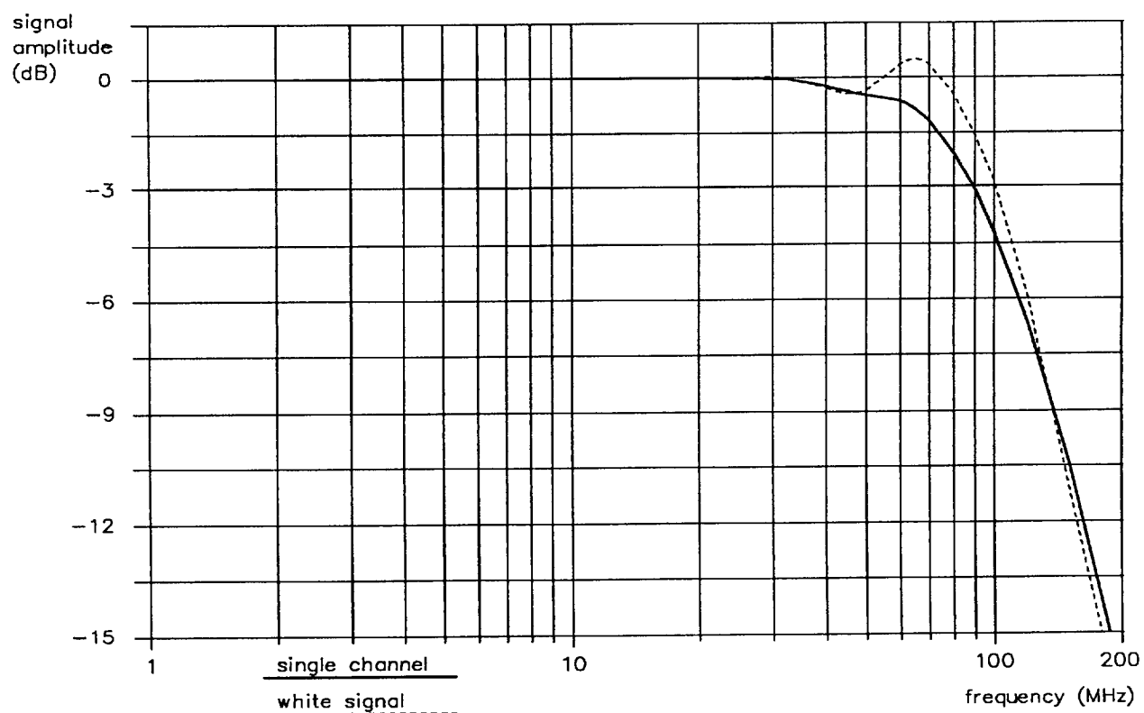
Fig.10 Typical frequency response.
