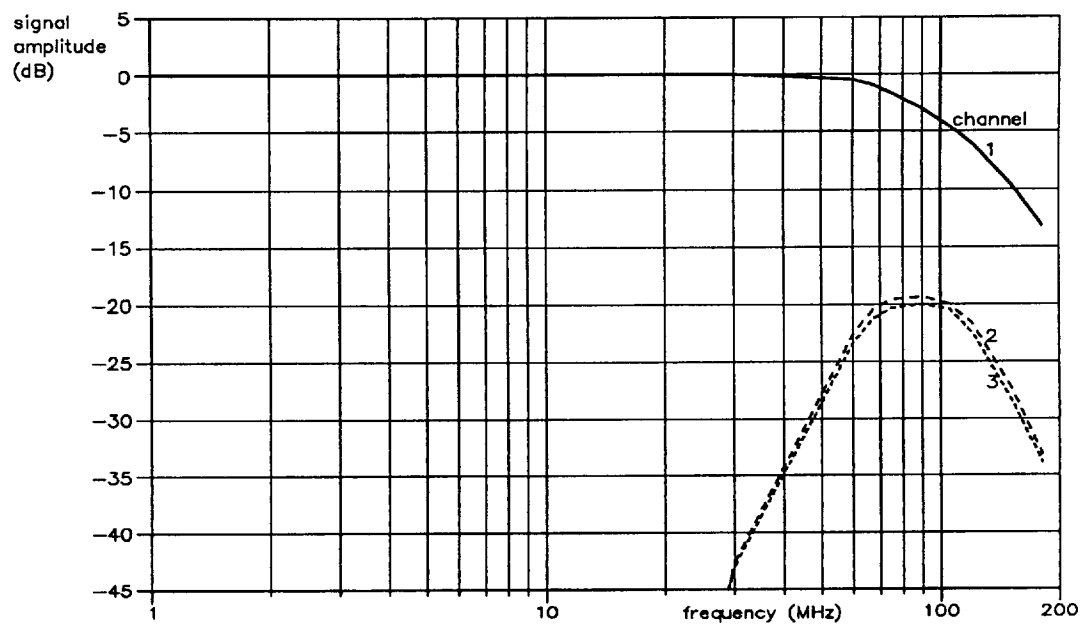
Fig.13 Typical crosstalk: Channel 1 → 2 and 3.
