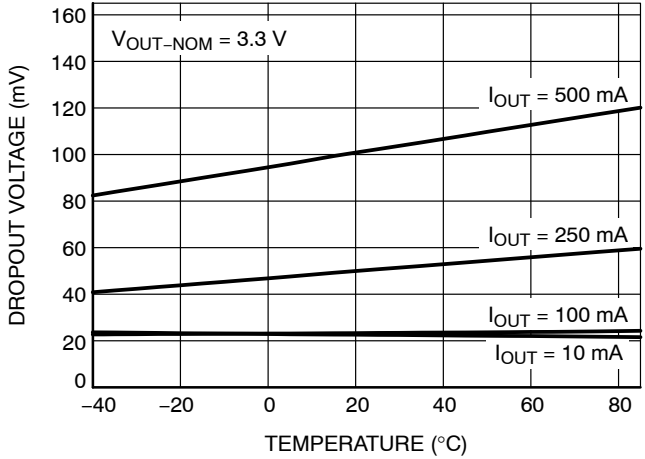
Figure 11. Dropout Voltage vs. Temperature
