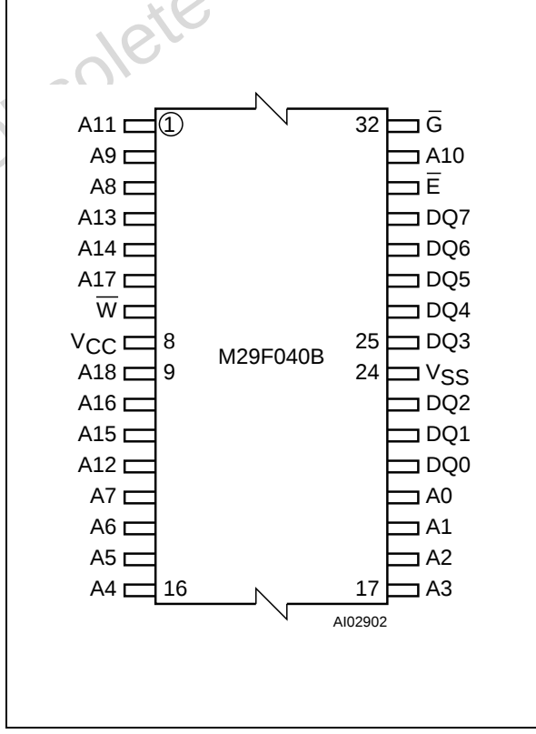
Figure 3. TSOP Connections
