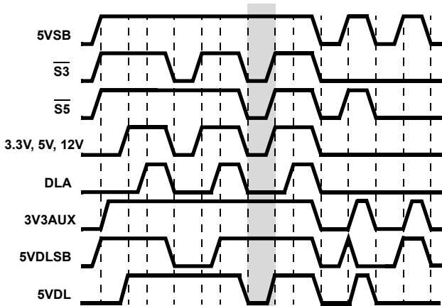
FIGURE 1. 5V DUAL AND 3.3V AUX TIMING DIAGRAM; ISL6506B
