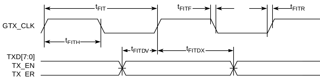
Figure 6. FIFO Transmit AC Timing Diagram
