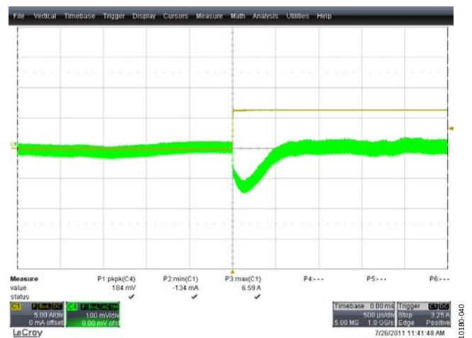
Figure 41. Output Voltage Transient, 0% to 25% Load, 385 V DC, One Phase Only Yellow Trace: Load Current, 5 A/div, 500 \mu s/div Green Trace: Output Voltage (AC-Coupled), 100 mV/div, 500 \mu s/div
