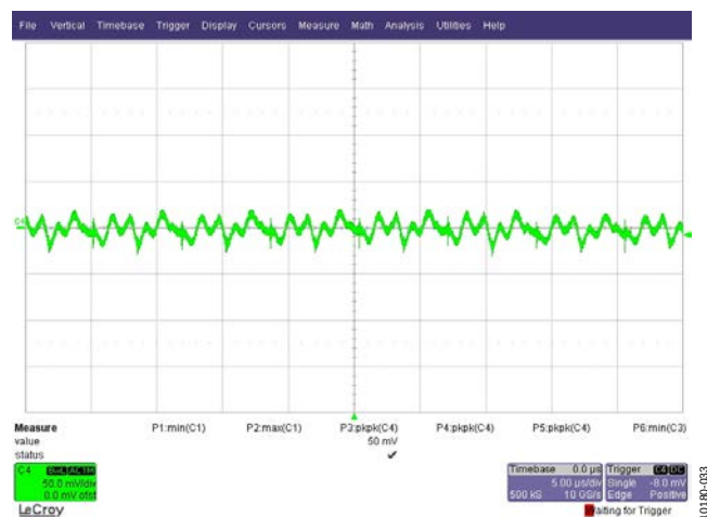
Figure 34. Output Voltage at C65 (AC-Coupled), 350 V DC, 25 A, 50 mV/div, 5 μs/div, High Frequency Component
