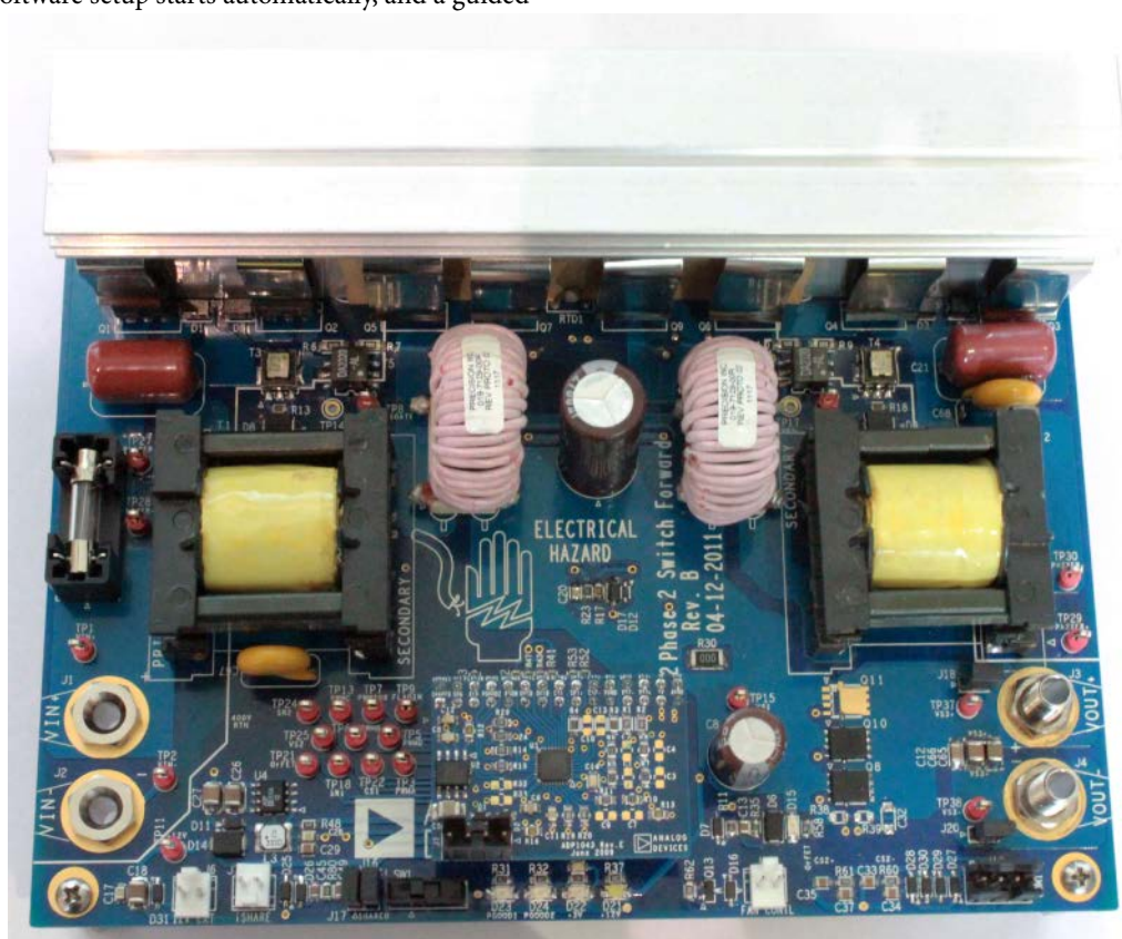
Figure 6. Printed Circuit Board with Daughter Card
