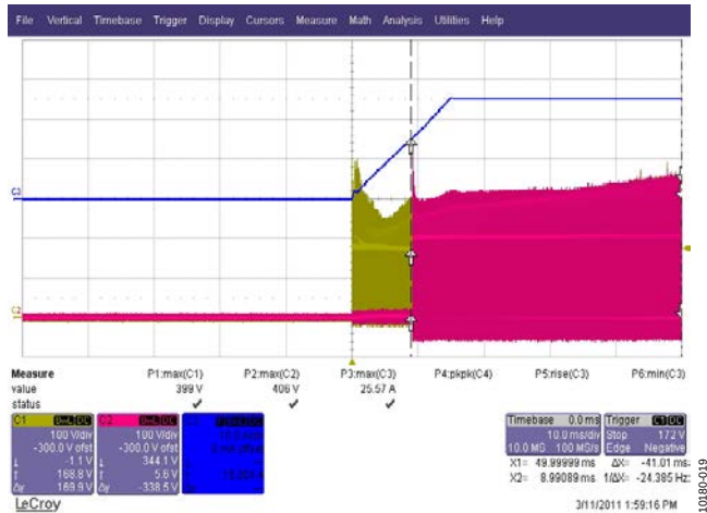
Figure 20. Startup at 385 VDC, Load (1 A/μs Slew Rate) Yellow Trace: Phase 1 Drain Voltage on Q2, 100 V/div, 10 ms/div Red Trace: Phase 2 Drain Voltage on Q4, 100 V/div, 10 ms/div Blue Trace: Load Current, 10 A/div, 10 ms/div Cursor Showing Phase 2 Enabled at 15 A
