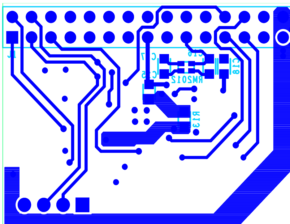
Figure 87. Bottom Layer, 1.5 in × 1.08 in
