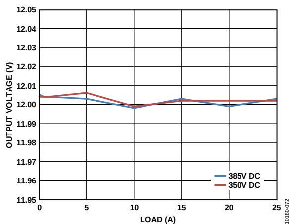
Figure 73. Output Voltage Regulation vs. Load Current
