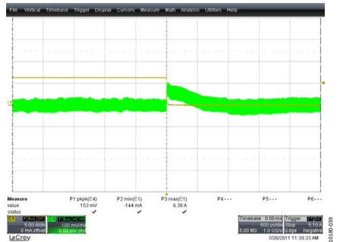
Figure 40. Output Voltage Transient, 25% to 0% Load, 385 V DC, Both Phases Active Yellow Trace: Load Current, 5 A/div, 500 \mu s/div Green Trace: Output Voltage (AC-Coupled), 100 mV/div, 500 \mu s/div
