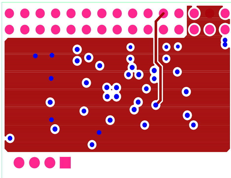
Figure 86. Power Layer, 1.5 in × 1.08 in
