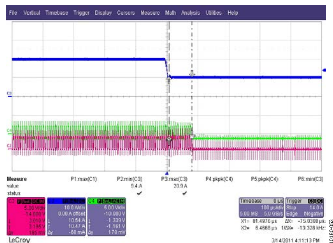
Figure 54. Synchronous Rectifier PWM Turn-On Time During Load Step 20 A to 10 A Load, Blue Trace: Load Current, 10 A/div, 100 μs/div Green and Red Trace: Phase 2 Synchronous Rectifier and Freewheel PWMs (SR1 and SR2), 100 μs/div
