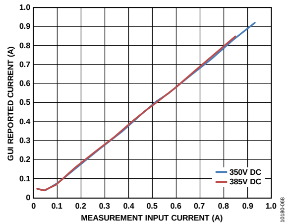
Figure 69. CS1 Linearity
