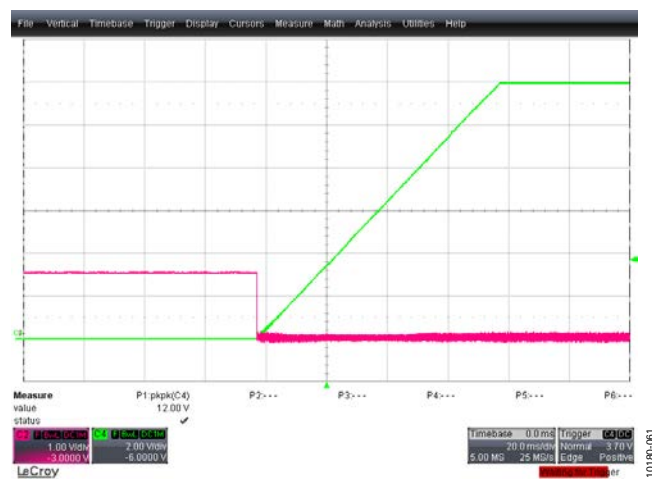
Figure 62. OrFET Turn-On Green Trace: Output Voltage, 2 V/div, 20 ms/div Red Trace: GATE Signal Voltage, 2 V/div, 20 ms/div
