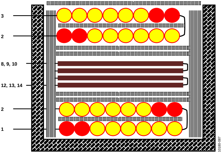
Figure 89. Transformer Construction Diagram
