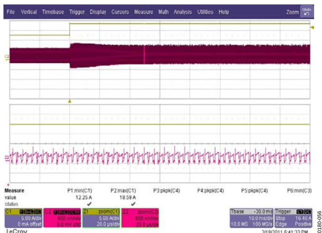
Figure 57. Input Current During Load Step of 10 A to 20 A Showing Steady Balancing of Both Phases; Yellow Trace: Load Current, 5 A/div, 10 ms/div Red Trace: Voltage at CS1 Pin, 500 mV/div (20 \mu s/div Zoomed In)
