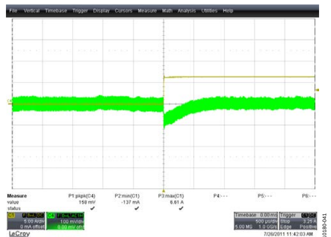
Figure 42. Output Voltage Transient, 0% to 25% Load, 385 V DC, Both Phases Active Yellow Trace: Load Current, 5 A/div, 500 \mu s/div Green Trace: Output Voltage (AC-Coupled), 100 mV/div, 500 \mu s/div
