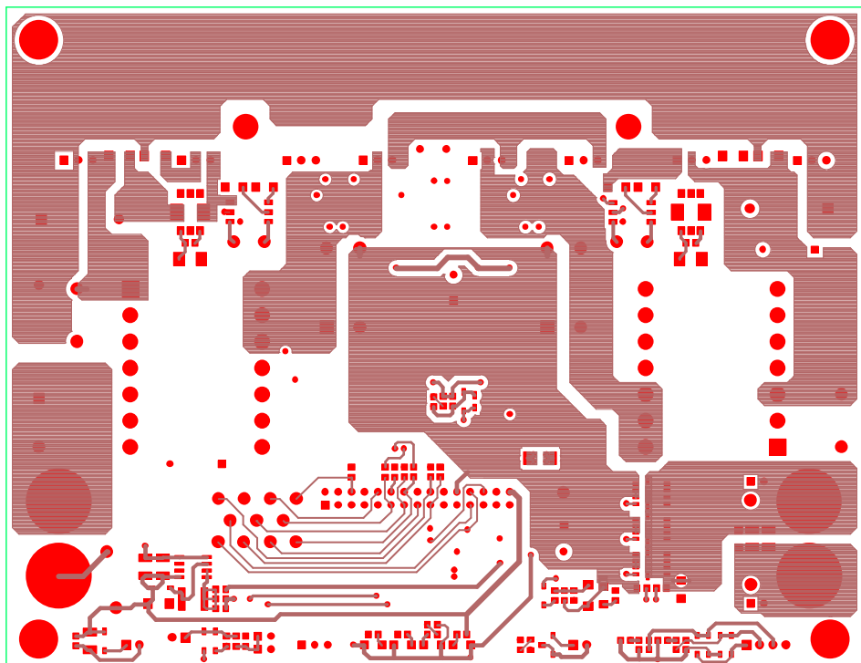
Figure 79. Layout, First Layer, 6.5 in x 5 in
