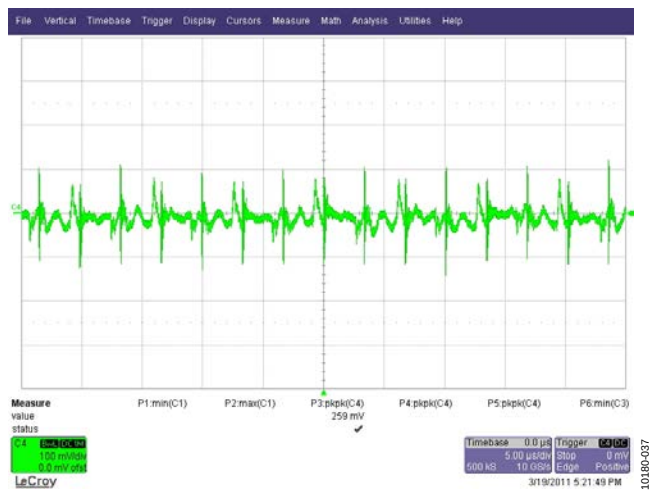
Figure 38. Output Voltage at 2700 \mu F Capacitor C10 (AC-Coupled), 385 V DC, 25 A, 100 mV/div, 5 \mu s/div, High Frequency Component
