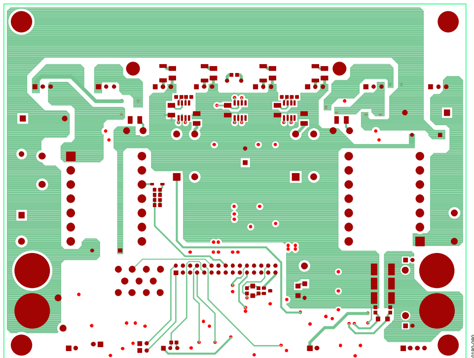
Figure 82. Layout, Bottom Layer, 6.5 in x 5 in
