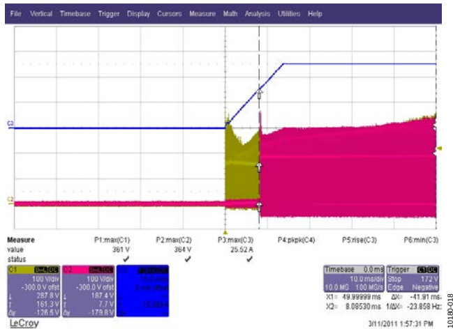
Figure 19. Startup at 350 VDC, Load (1 A/μs Slew Rate) Yellow Trace: Phase 1 Drain Voltage on Q2, 100 V/div, 10 ms/div Red Trace: Phase 2 Drain Voltage on Q4, 100 V/div, 10 ms/div Blue Trace: Load Current, 10 A/div, 10 ms/div Cursor Showing Phase 2 Enabled at 15 A
