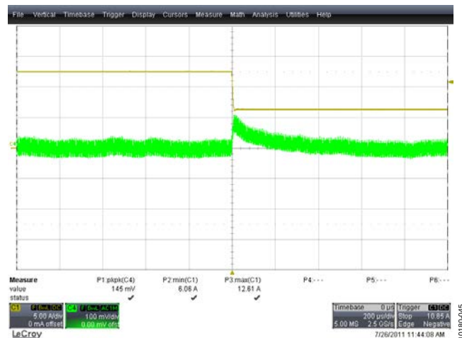
Figure 46. Output Voltage Transient, 50% to 25% Load, 385 V DC, Both Phases Active Yellow Trace: Load Current, 5 A/div, 200 \mu s/div Green Trace: Output Voltage (AC-Coupled), 100 mV/div, 200 \mu s/div
