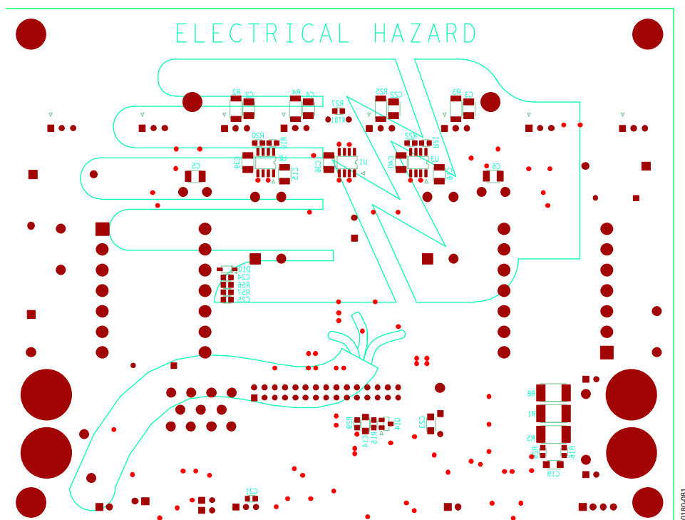
Figure 83. Layout, Bottom Layer Silkscreen, 6.5 in x 5 in
