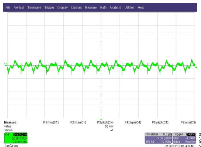
Figure 36. Output Voltage at C65 (AC-Coupled), 385 V DC, 25 A, 50 mV/div, 5 μs/div, High Frequency Component
