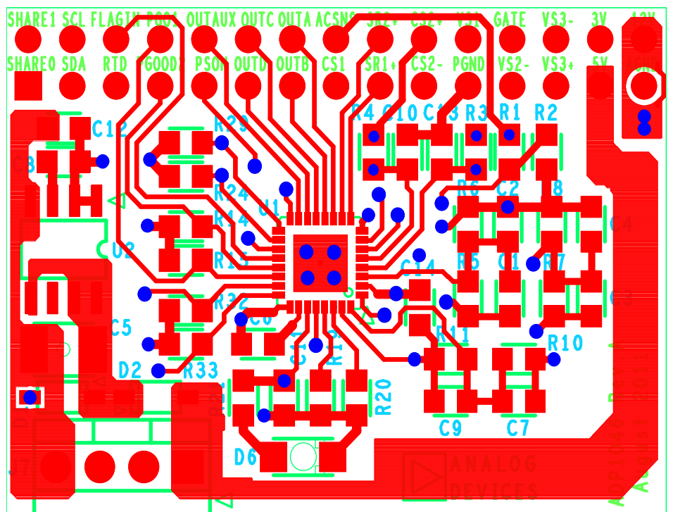
Figure 84. Top Layer, 1.5 in × 1.08 in
