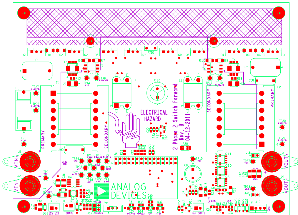
Figure 78. Layout, Top Silkscreen, 6.5 in x 5 in
