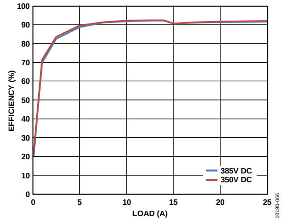
Figure 67. Efficiency vs. Load
