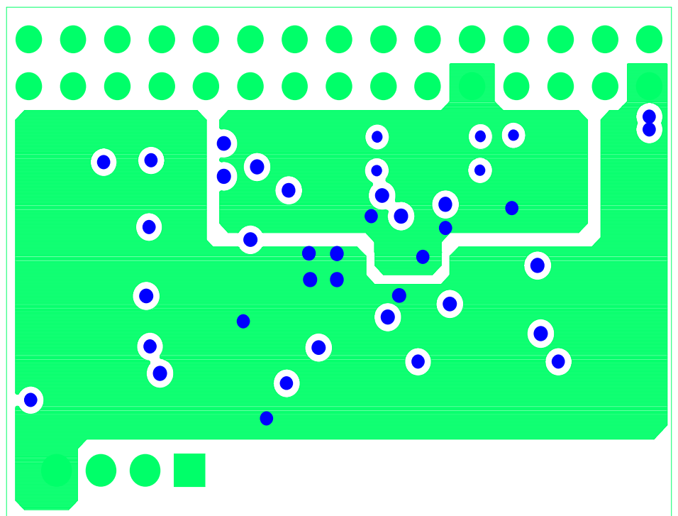
Figure 85. Ground Layer, 1.5 in × 1.08 in
