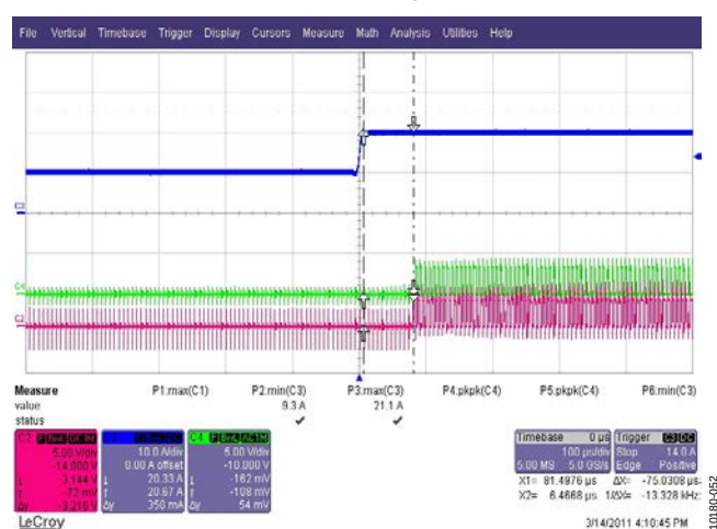
Figure 53. Synchronous Rectifier PWM Turn-On Time During Load Step 10 A to 20 A Load, Blue Trace: Load Current, 10 A/div, 100 μs/div Green and Red Trace: Phase 2 Synchronous Rectifier and Freewheel PWMs (SR1 and SR2), 100 μs/div
