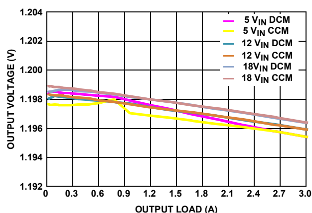
FIGURE 10. V_{OUT} REGULATION vs LOAD, 1.2V
