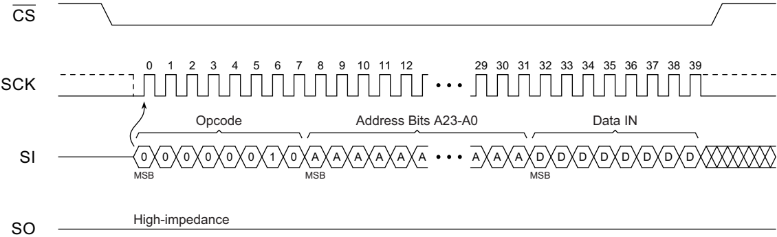
Figure 8-1. Byte Program
