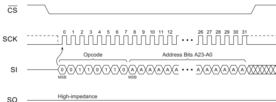
Figure 9-3. Protect Sector
