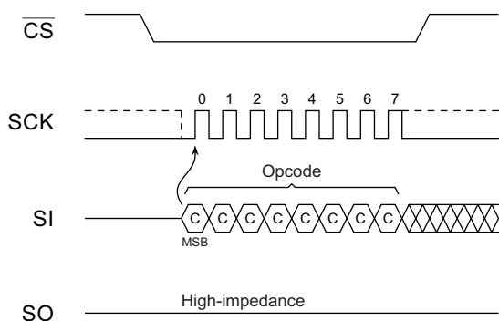
Figure 8-8. Chip Erase
