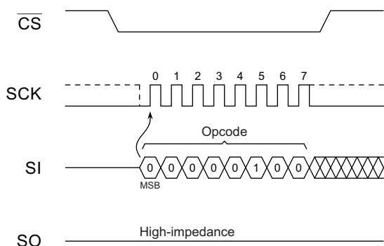
Figure 9-2. Write Disable
