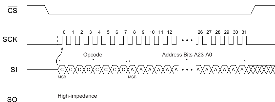
Figure 8-7. Block Erase
