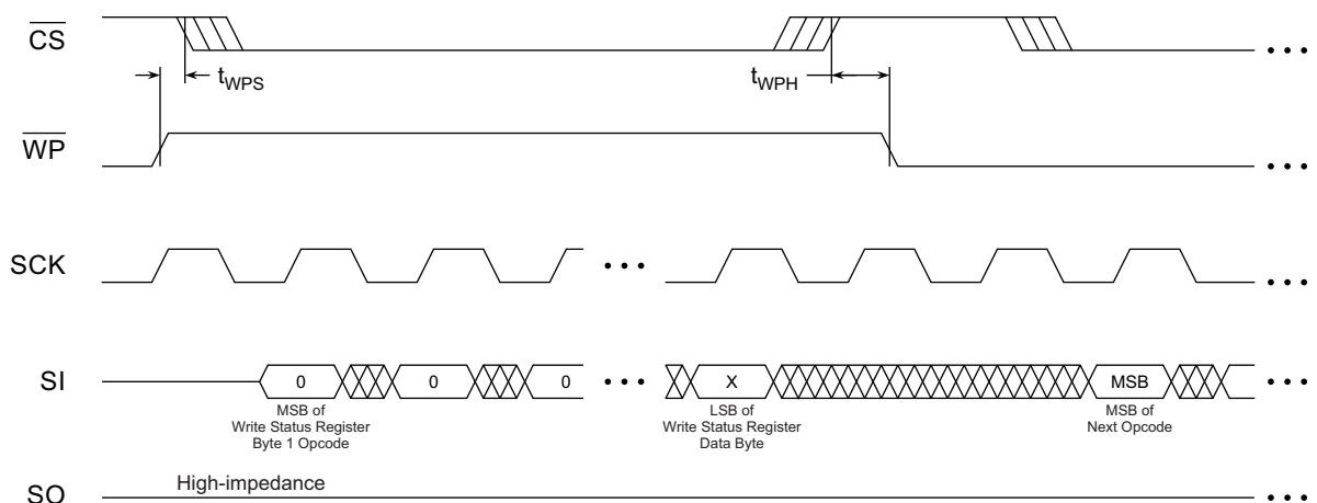
Figure 14-3. \overline{\text{WP}} Timing for Write Status Register Byte 1 Command When SPRL = 1
