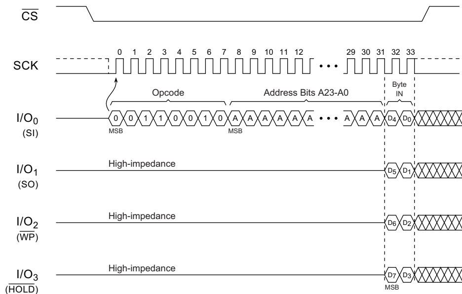
Figure 8-5. Quad-Input Byte Program
