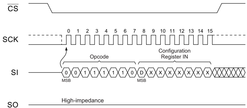
Figure 11-5. Write Configuration Register
