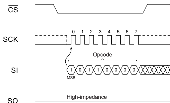
Figure 8-9. Program/Erase Suspend
