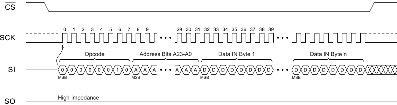
Figure 8-2. Page Program
