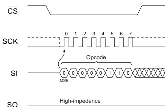
Figure 9-1. Write Enable
