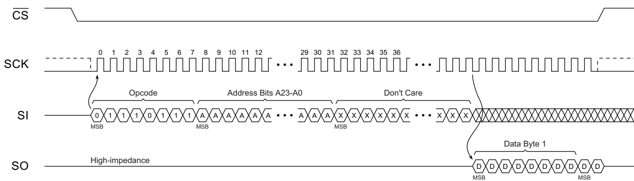
Figure 10-5. Read OTP Security Register
