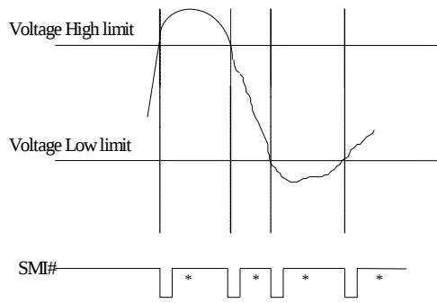
Figure 15-1. Voltage SMI# Mode
