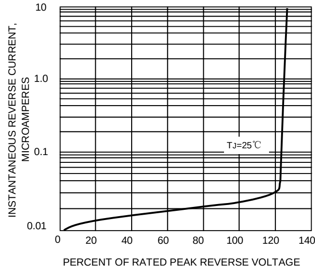
FIG.3-TYPICAL REVERSE CHARACTERISTICS
