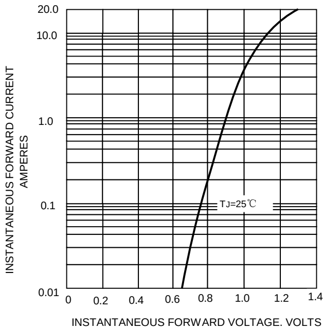
FIG.2-TYPICAL FORWARD CHARACTERISTICS
