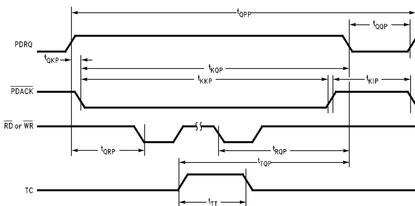
FIGURE 10-12b. ECP DMA Timing
