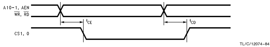
FIGURE 10-27. Chip Select Timing
