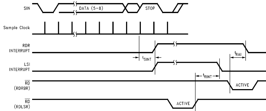
FIGURE 10-8. Receiver Timing
