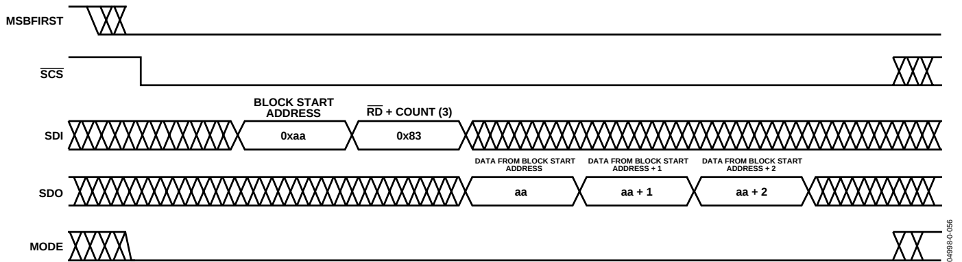
Figure 47. Serial Read of Three Bytes with \text{MSB\_FIRST} = 0 (All Words are Written or Read LSB First)
