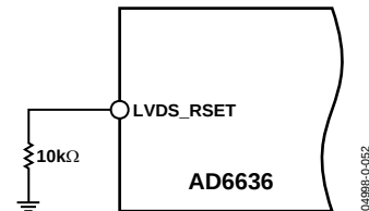
Figure 60. LVDS_RSET Circuit for LVDS Calibration
