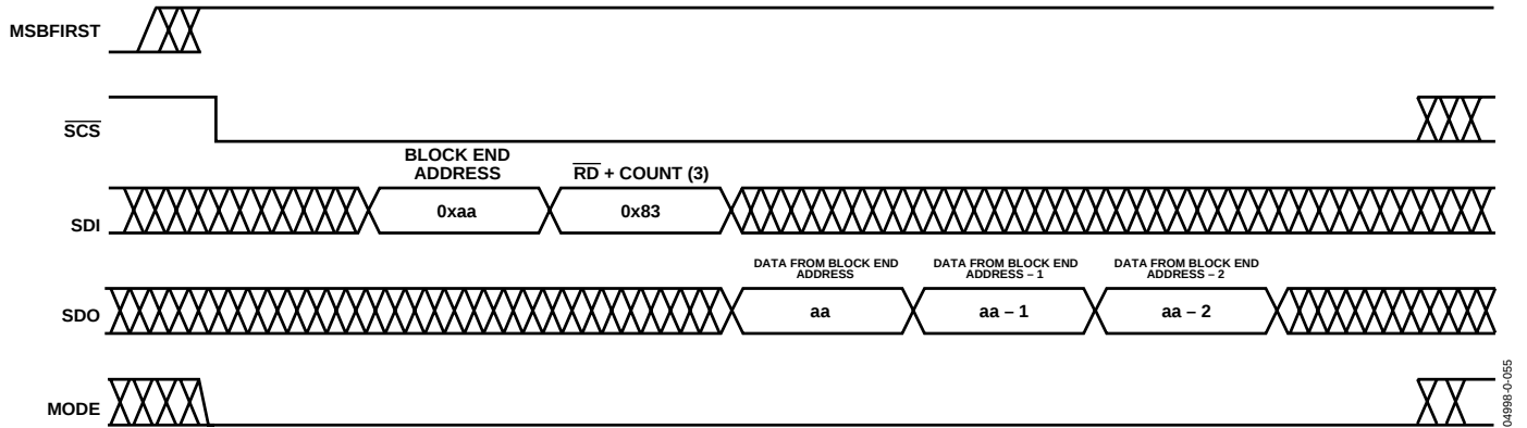
Figure 46. Serial Read of Three Bytes with \text{MSB\_FIRST} = 1 (All Words are Written or Read MSB First)
