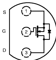
Top View VN0808LS
