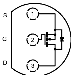
Top View VN0808L
