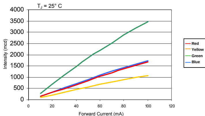
Intensity vs Forward Current
