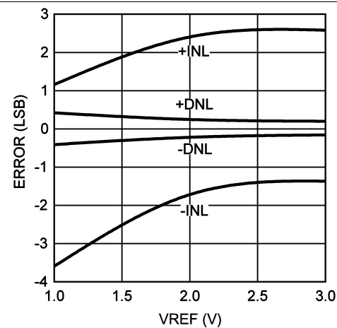
Figure 7. INL/DNL vs V_{REF} at V_A = 3 V
