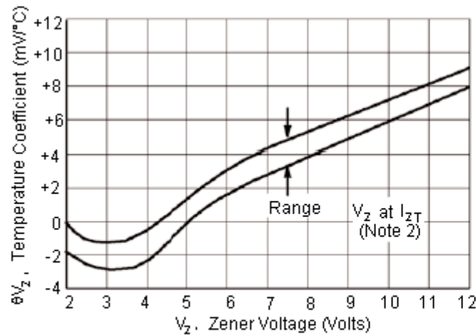
Temperature Coefficients
