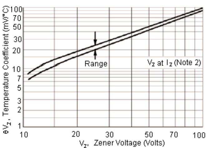
Temperature Coefficients
