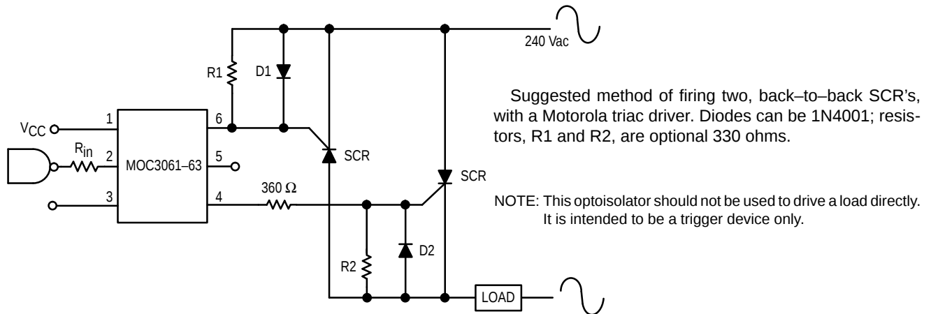
Figure 9. Inverse-Parallel SCR Driver Circuit
