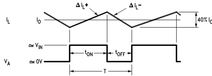
Figure 23. Relation of Switch Timing to Inductor Current in Step-Down Regulator
