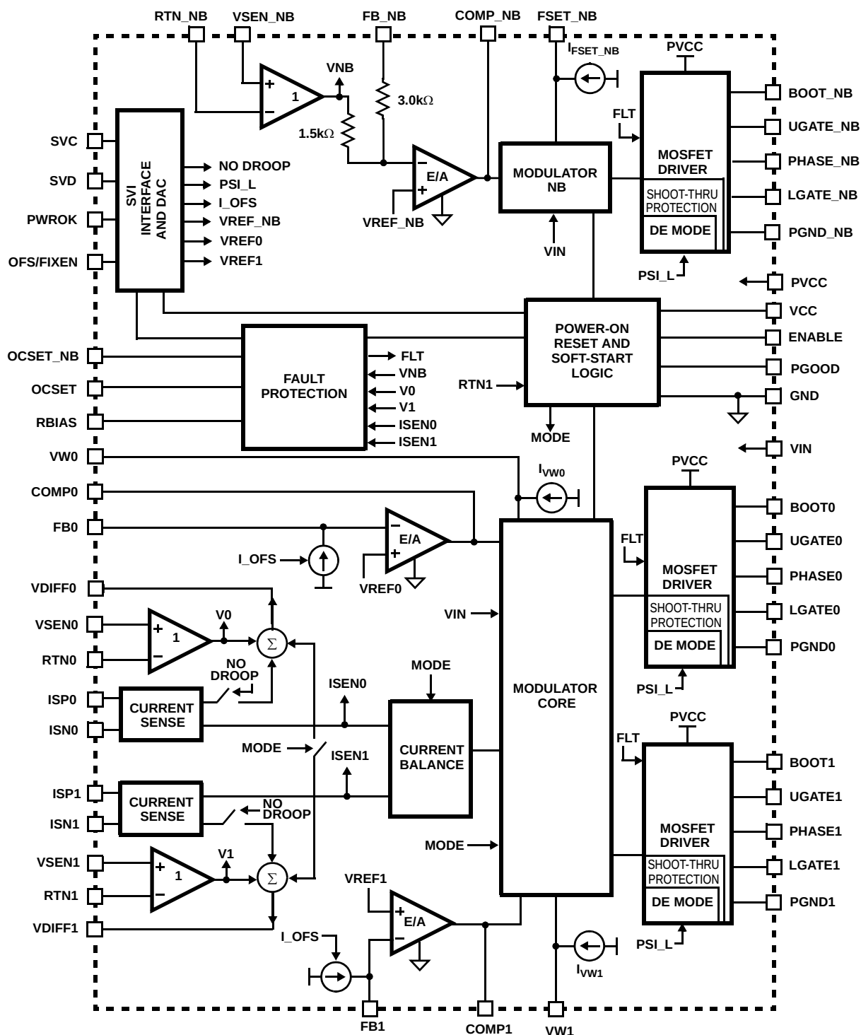
FIGURE 1. SIMPLIFIED FUNCTION BLOCK DIAGRAM OF ISL6265
