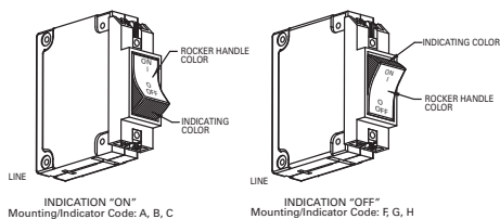
MARKING DETAIL "A" (SEE TABLE)
