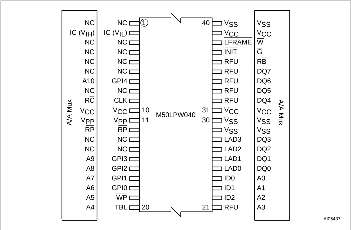
Figure 3. TSOP Connections
