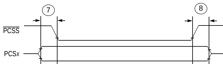
Figure 24. DSPI PCS Strobe ( \overline{\text{PCSS}} ) Timing
