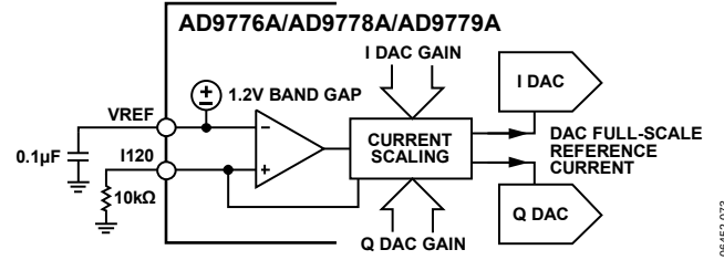
Figure 76. Reference Circuitry
