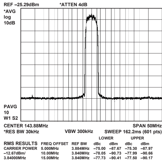
Figure 49. AD9776A Single Carrier W-CDMA, 4\times Interpolation, f_{DATA} = 122.88 \text{ MSPS} , Amplitude = -3 dBFS
