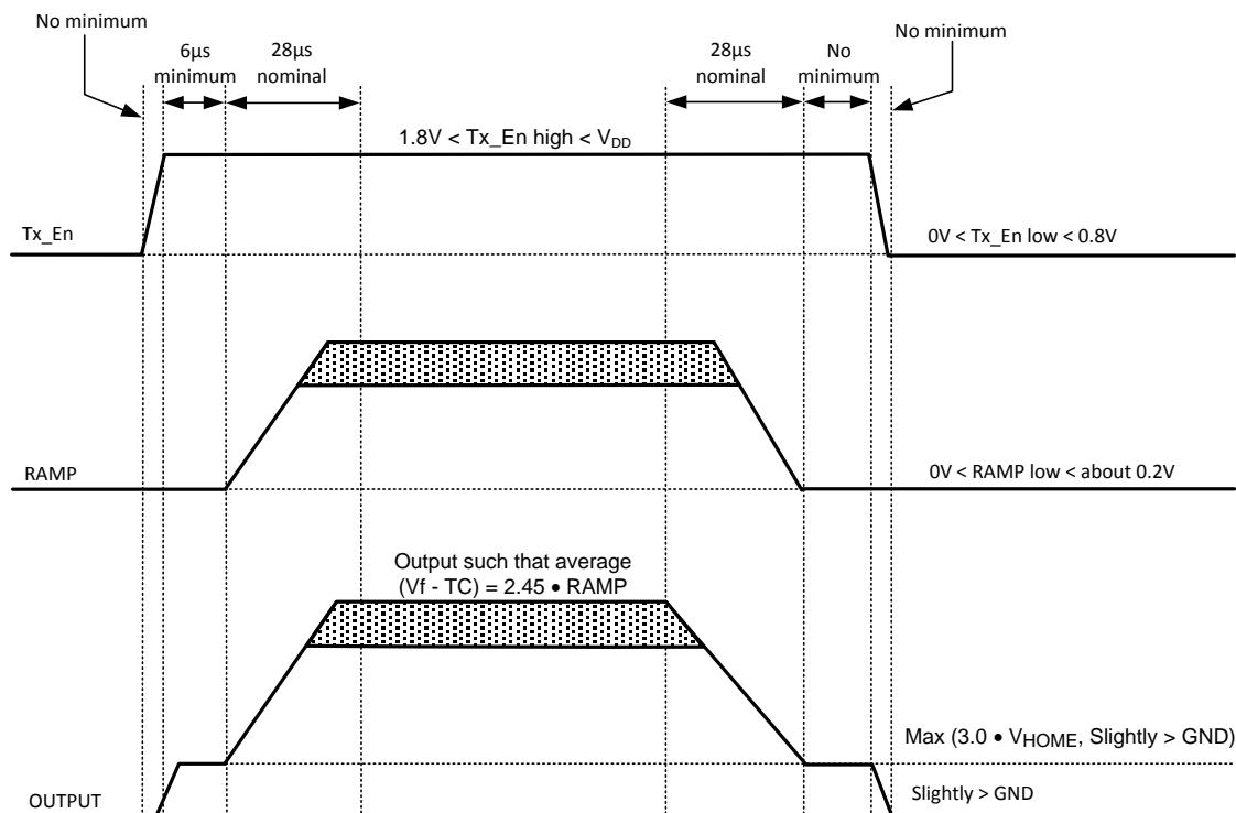
Timing Diagram #2 Tx/Rx Enabled
