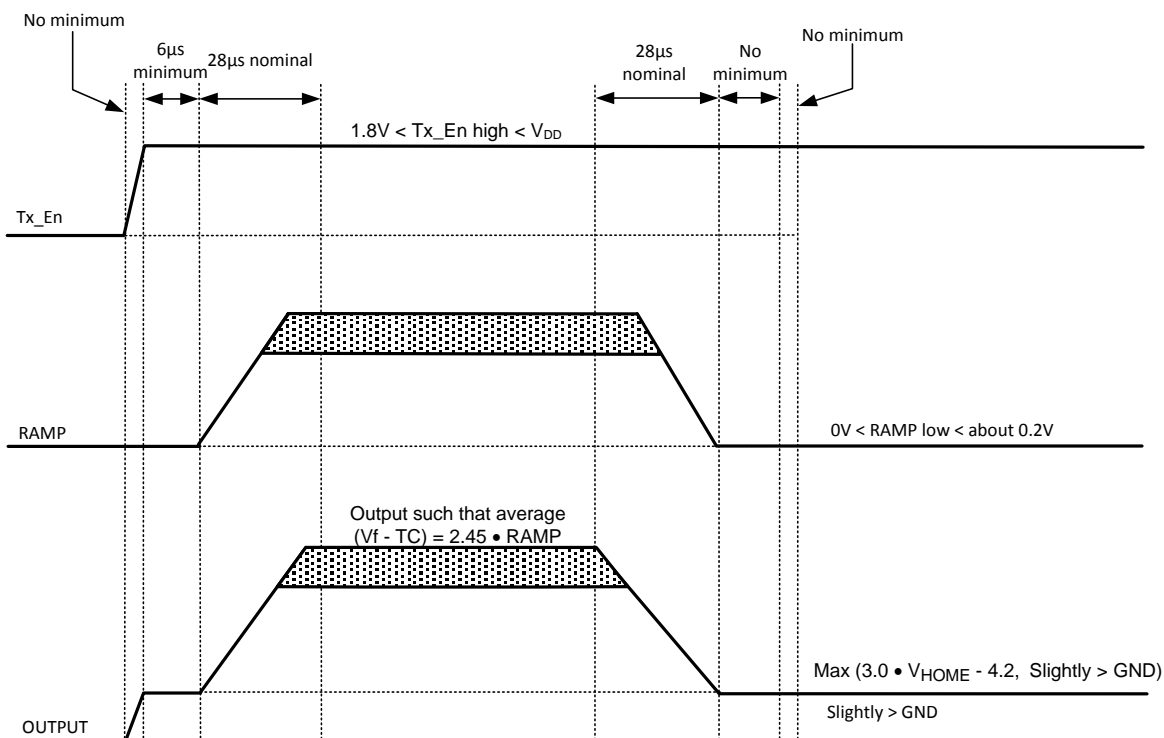
Timing Diagram #2 Tx/Rx Enabled
