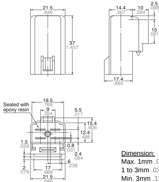
External dimensions
