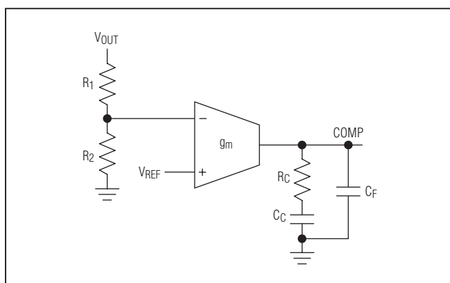
Figure 3. Compensation Network
