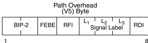
Figure 2. 1544 kbit/s Mapping
