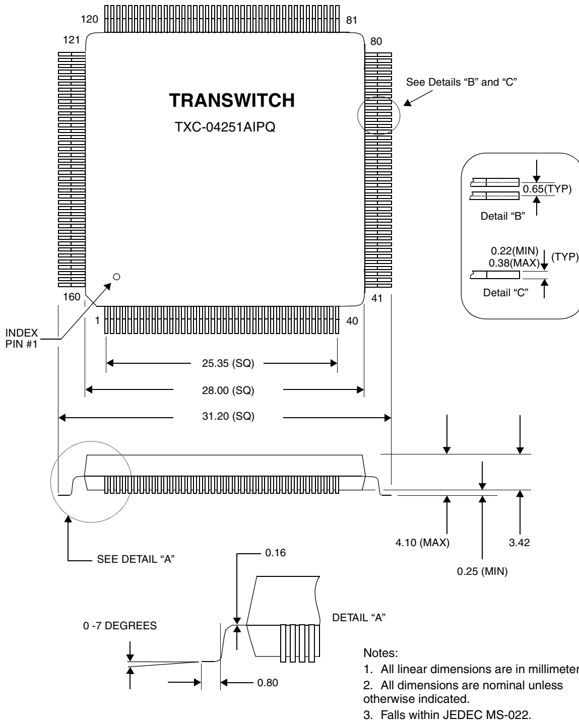
Figure 17. QT1M TXC-04251 160-Pin Plastic Quad Flat Package
