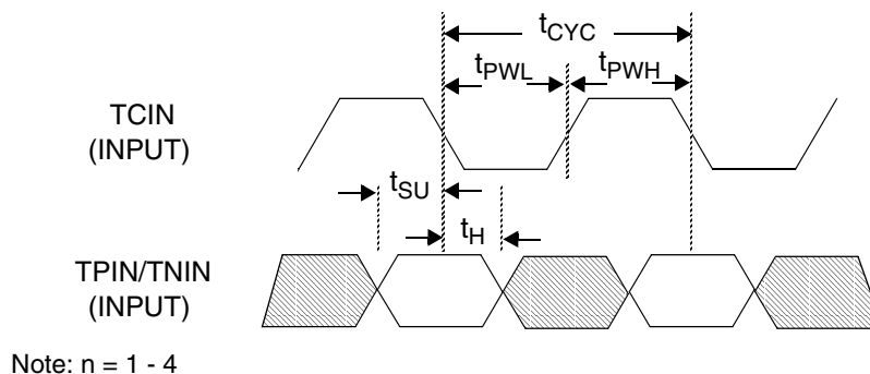
Figure 4. Ports 1, 2, 3 and 4 DS1 Transmit Timing
